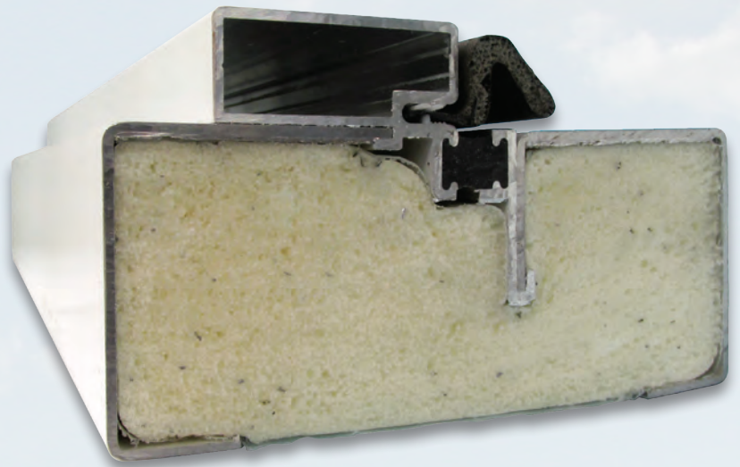
■ Optional Foam-Injected Insulated Frame
